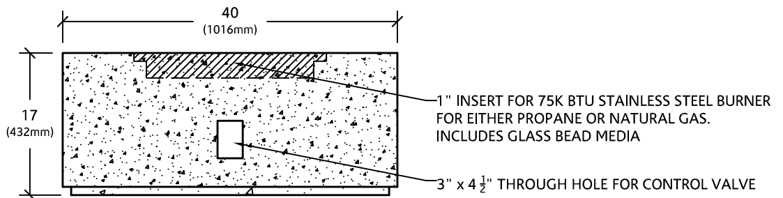
ELEVATION VIEW
